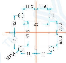
Installation hole figure
