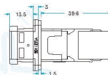
S socket (dimensions figure)
