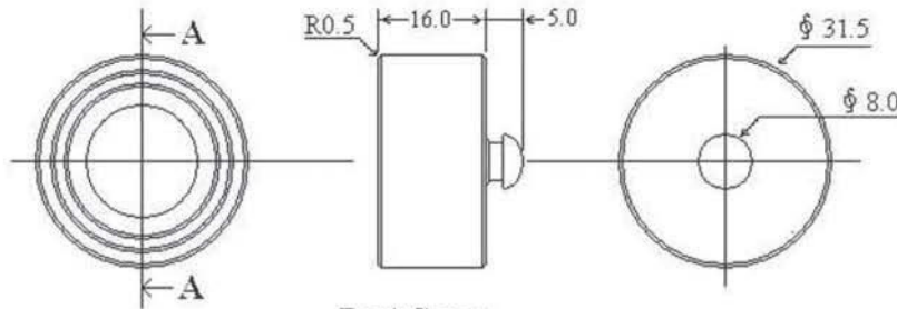
Dust Cover Material EPDM Black
