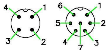
Pin Assignment Front View (前視圖)
