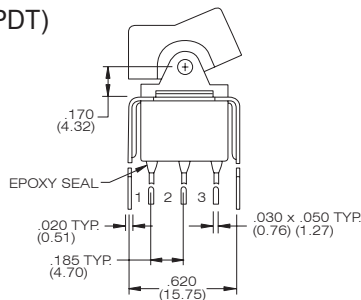
NER8015-R11-2-CQ-S20
