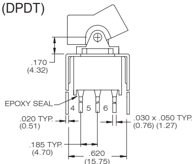
NER8017 - R11-2-CQ-S20
