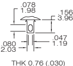
THK 0.76 (.030)
