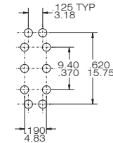
P.C. MOUNTING
