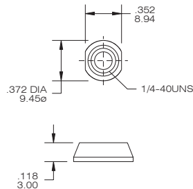
DRESS NUT
