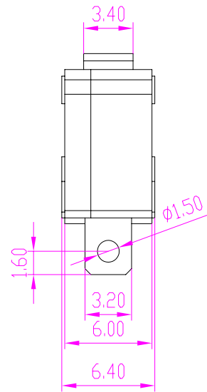
Mounting hole dimensions
