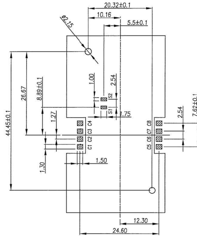
Reference dimension for PCB layout
