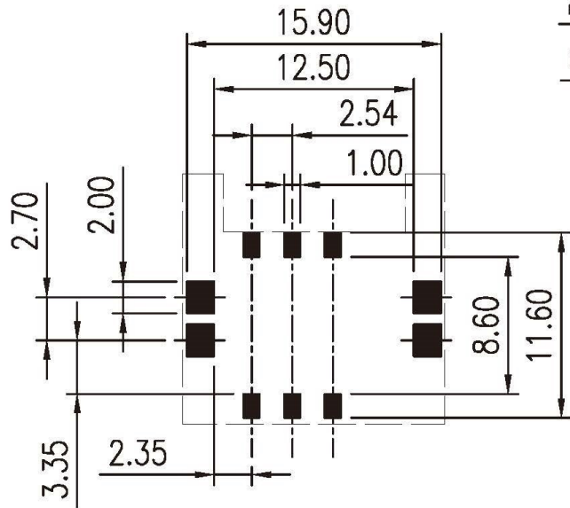
Recommended P.C.B. Layout (Tolerance = \pm 0.05 ) AS VIEW FROM COMPONENT SIDE
