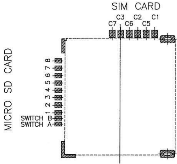
CIRCUIT POSITION
