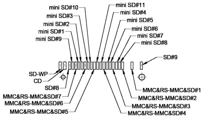
GROUND X2 PCB LAYOUT
