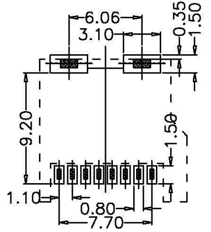
RECOMMENDED P.C.B HOLE LAYOUT COMPONENT SIDE VIEW(TOLERANCE: +/-0.05)
