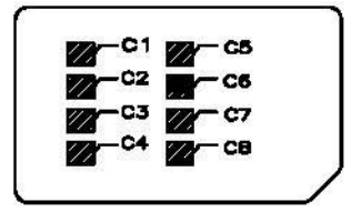
REFERENCE SIM CARD PLUG
