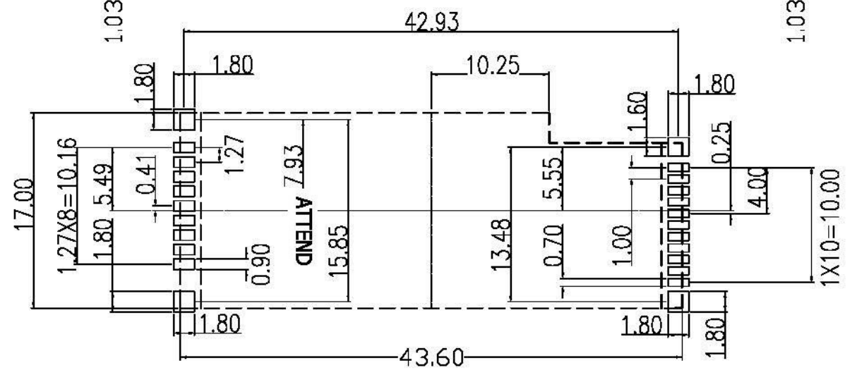
RECOMMENDED PCB LAYOUT TOL:(±0.05)
