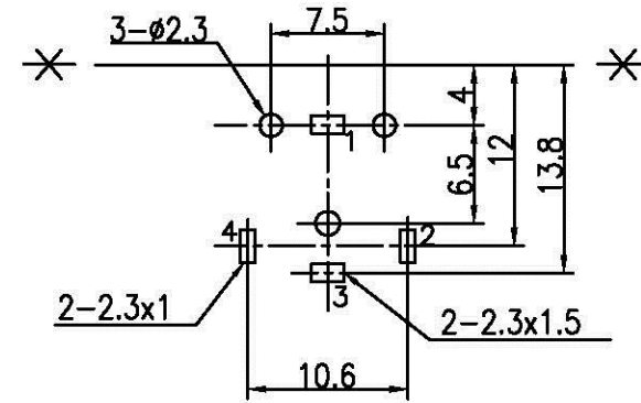
T:1.6 Dimensions of PC board holes Tolerance : ±0.1(Printed-side view)
