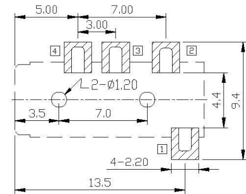
RECOMMENDED SOLDER PAD LAYOUT (±0.1)
