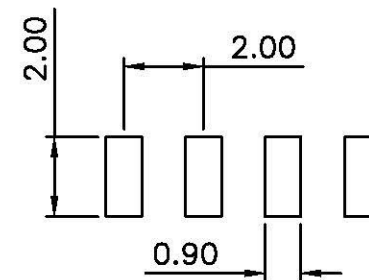
Recommended P.C.Board
