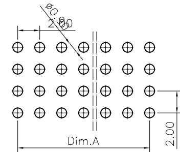
Recommended P.C.B. Layout (Tolerance: 0.05mm)
