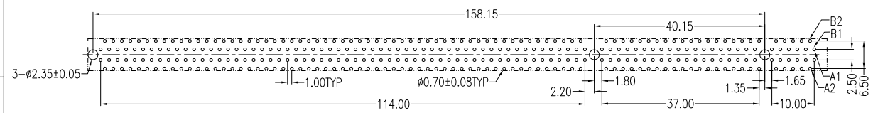
PCB LAYOUT Top View
