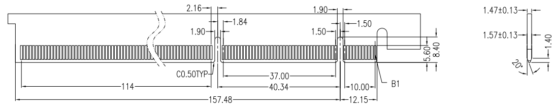
DAUGHTER CARD PRIMARY (COMPONENT) SIDE
