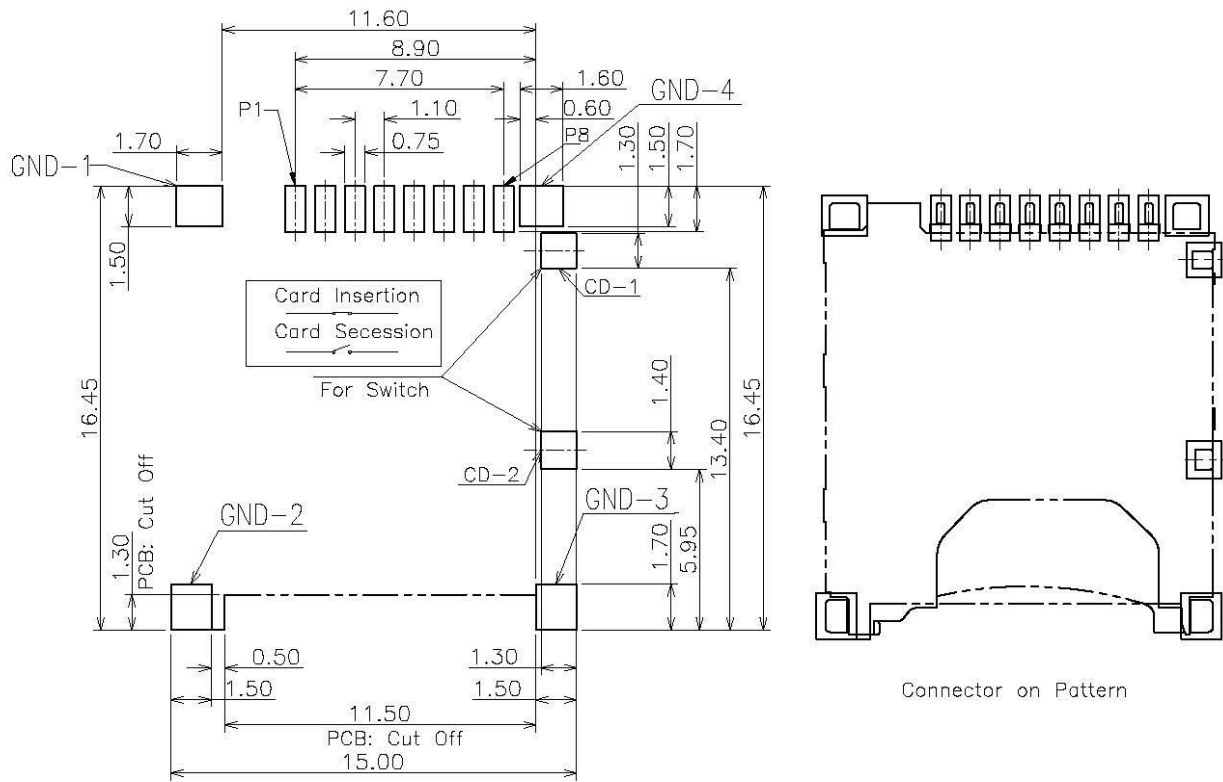
Recommended PCB Pattern Layout General Tolerance: ±0.05
