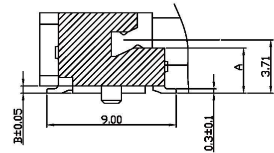
B-B' SECTION
