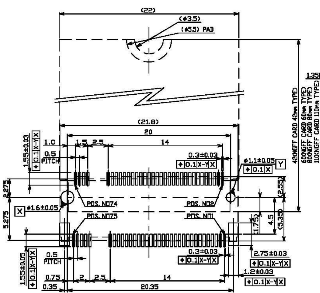
KEY ID "M" RECOMMENDED P.C.BOARD LAYOUT
