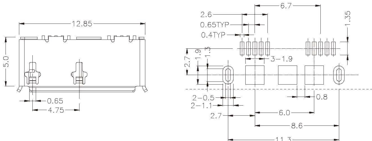
P.B.C LAYOUT TOP VIEW ±0.05
