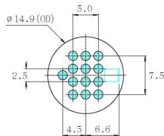
PIN LAYOUT
