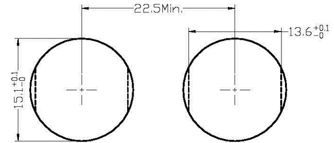
PANEL CUT-OUT
