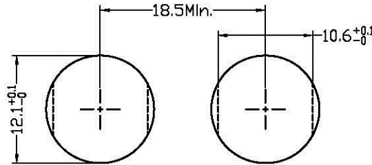
PANEL CUT-OUT
