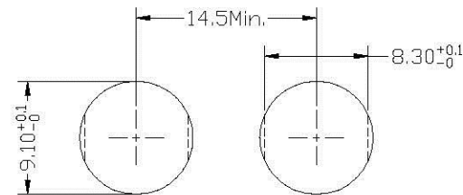
PANEL CUT-OUT
