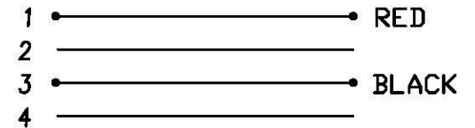
CON 1 PIN ASSIGNMENTS
