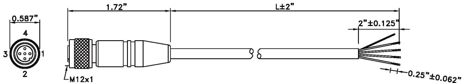
FRONT VIEW
