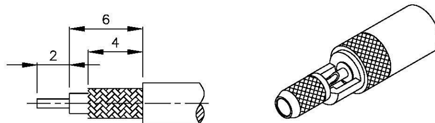
(Recommended Stripping Dimension)
