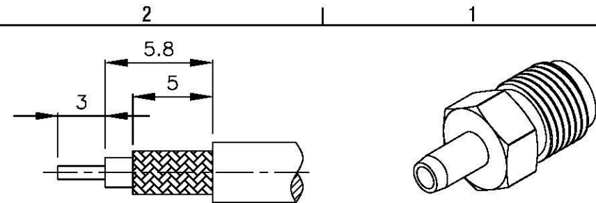
(Recommended Stripping Dimension)
