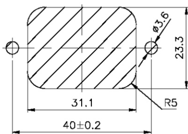
PANEL CUT-OUT
