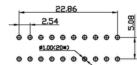
P. C. B LAYOUT (±0.05)
