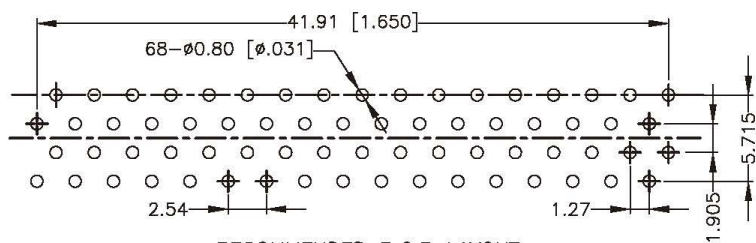
RECOMMENDED P.C.B LAYOUT TOLERANCE \pm 0.05 TOP VIEW
