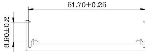
Strain Relief
