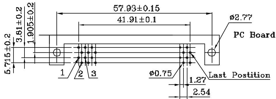
PC Board Mounting Dimensions
