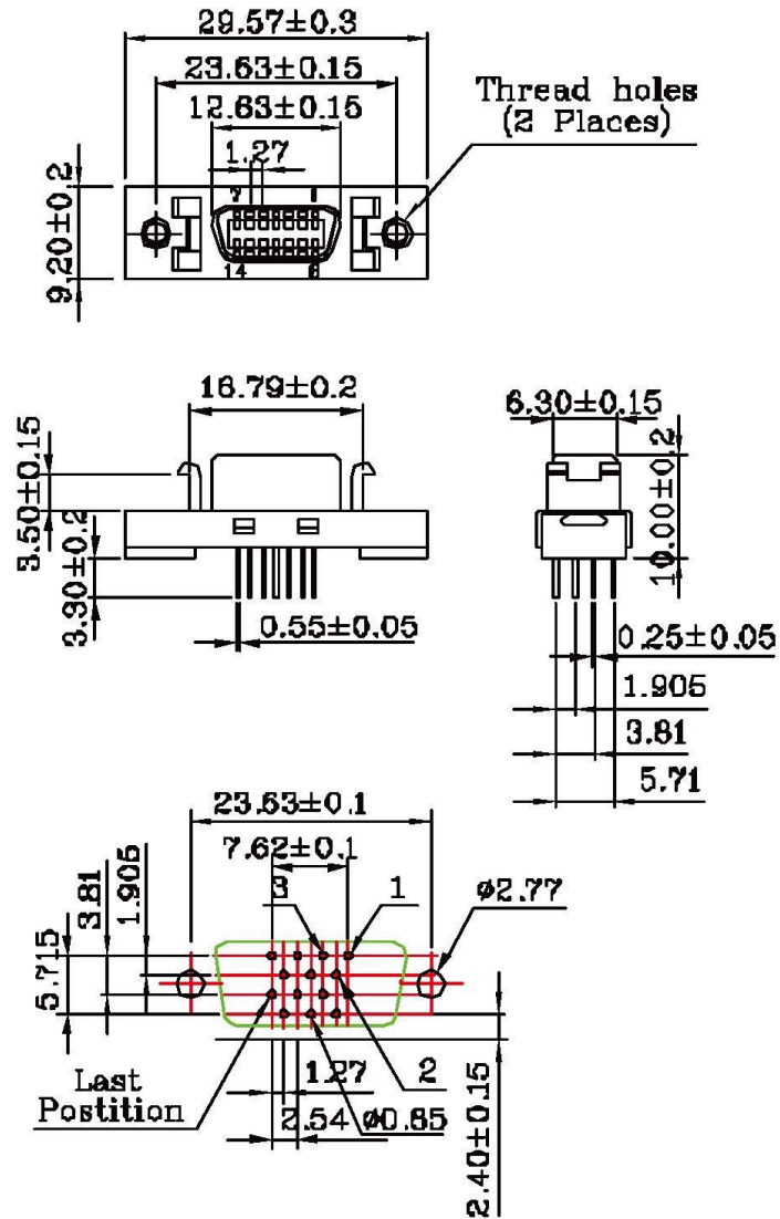
PC Board Mounting Dimensions
