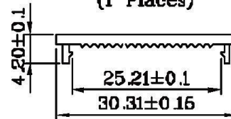
Termination Cover (1 Places)
