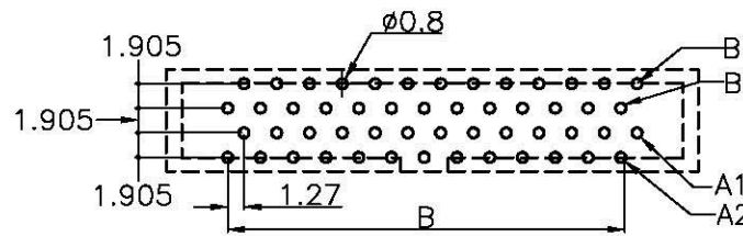
P.C. Board Layout Top View (Tolerance:±0.05) (20,32,40,52,60,68,80,100 Position)
