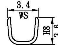
B-B Section
