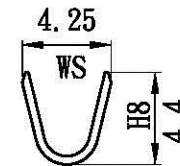
B-B Section
