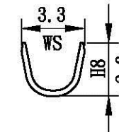
B-B Section
