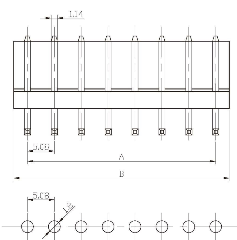
RECOMMENDED P.C.BOARD HOLE DIM.
