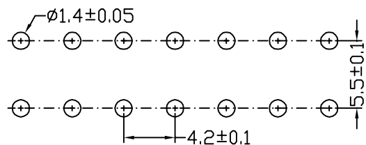
P.C.B. RECOMMENDED LAYOUT
