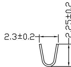
B-B SEC
