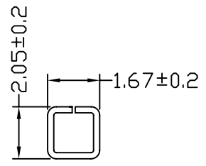
C-C SEC
