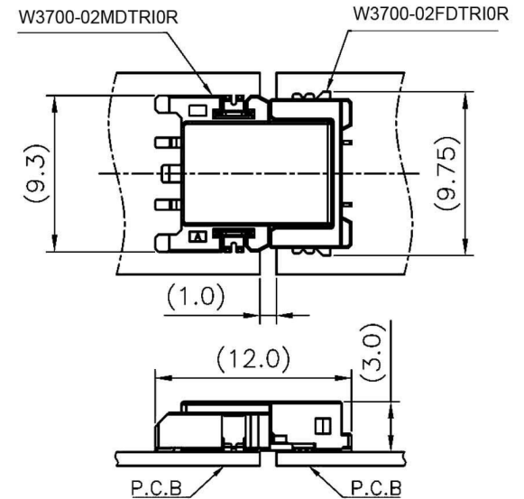
MATED CONNECTOR(REFERENCE)
