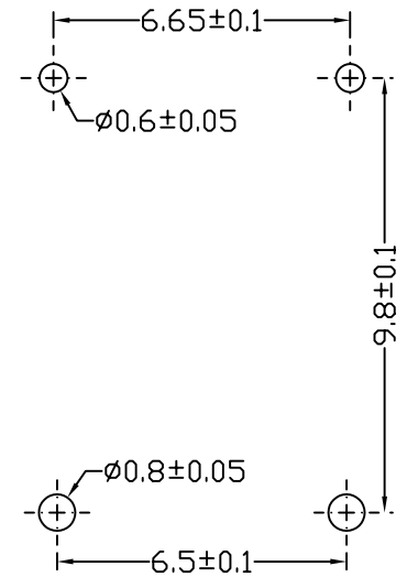
Recommend PCB Layout
