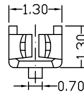
C-C SEC
