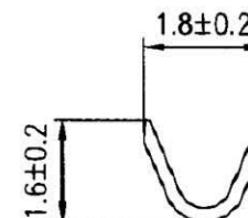
B-B SECTION
