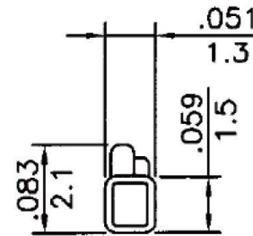
C-C SECTION
