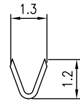
B-B SECTION
